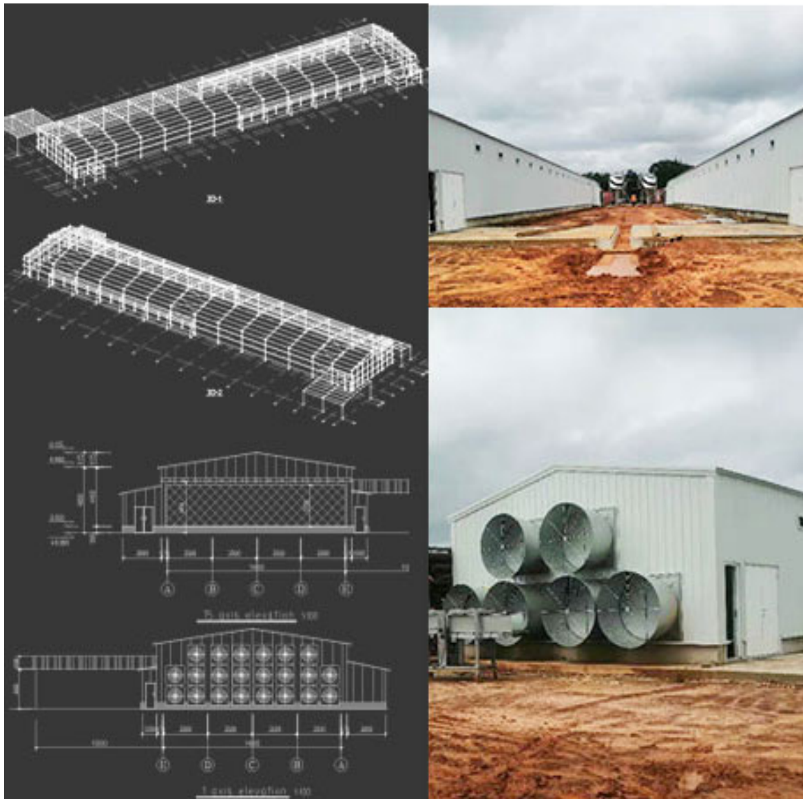
poultry house plans in Ghana
